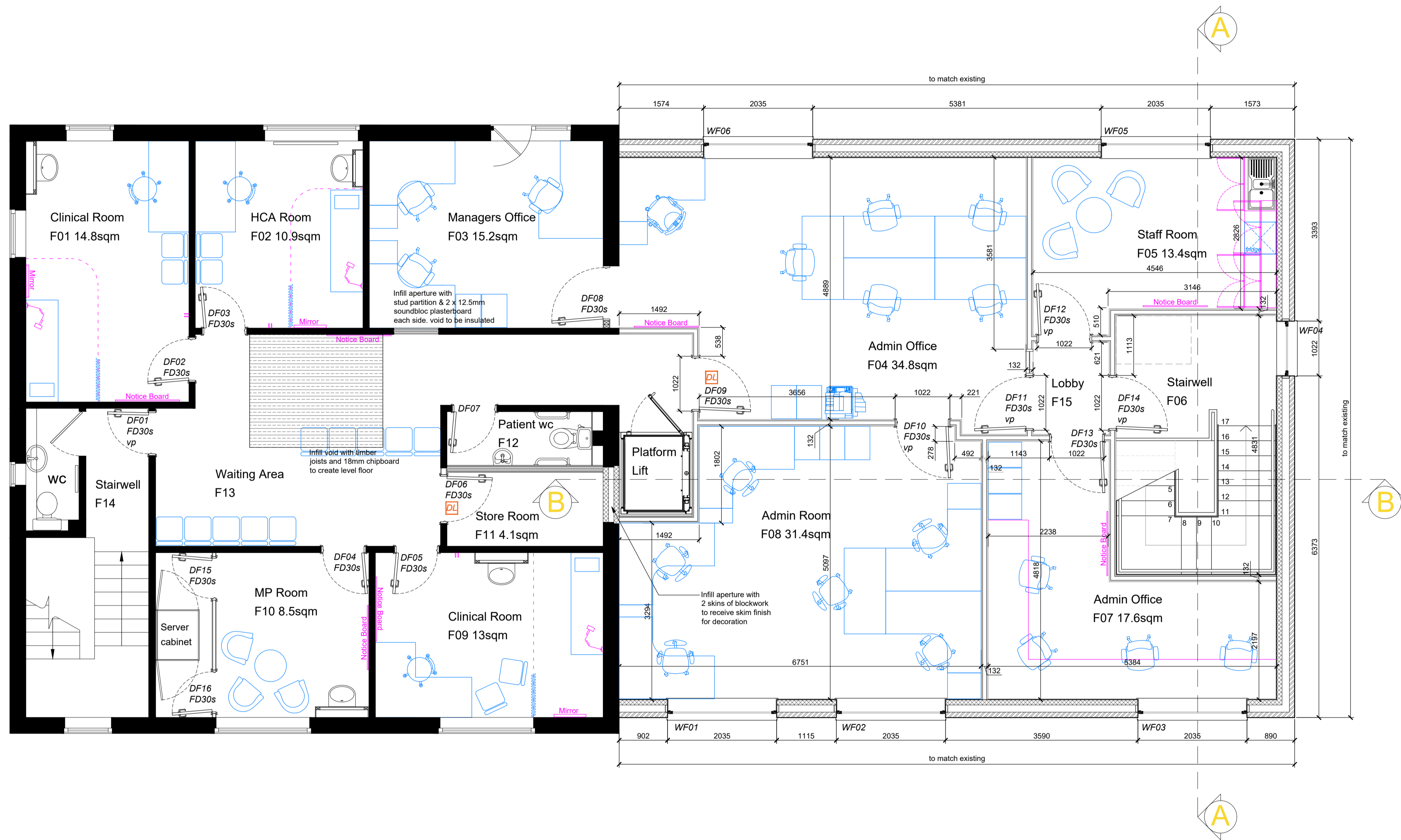
First Floor Proposed GA Plan 1:50 @ A1
